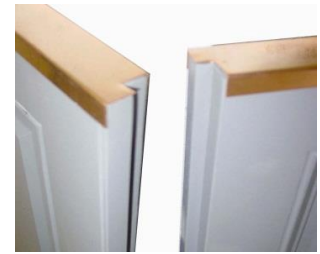
RABBET & BEAD OVERLAP (SHOWN WITH NOTCHED CAPS)
