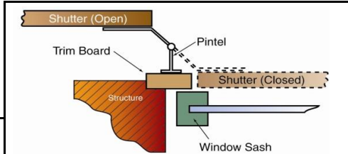
Frame Construction - Inside Mount
