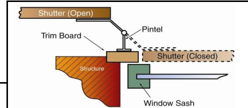
Frame Construction - Inside Mount
