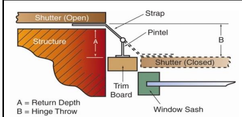
Brick Construction - Inside Mount
