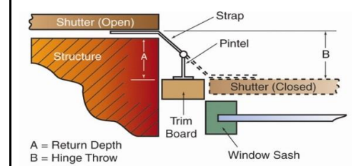
Brick Construction - Inside Mount
